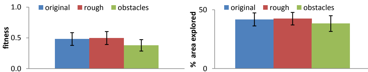
Fig. 5. Graphs showing average fitness (left) and exploration(right) of all evolutionary runs
